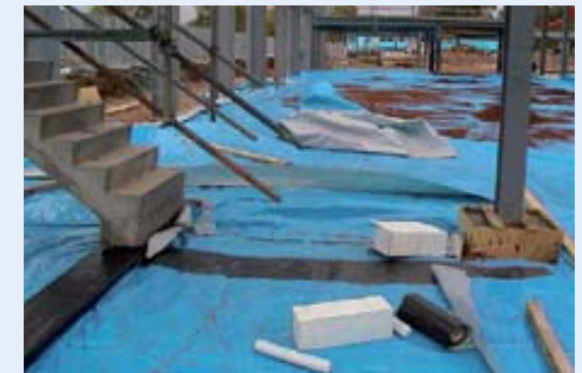
Make sure the root barrier membrane is sealed properly around pillars and other structures.
